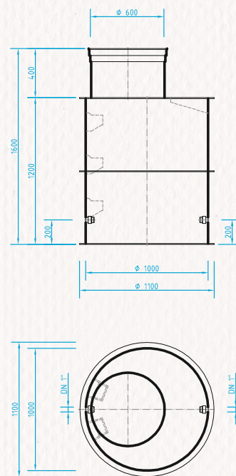
WATER SHAFT - CIRCULAR 2 \varnothing 1000 \times 1600 mm
