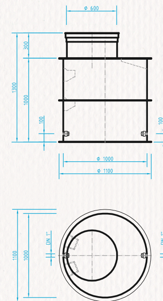
WATER SHAFT - CIRCULAR 4 \varnothing 1000 \times 1300 mm
