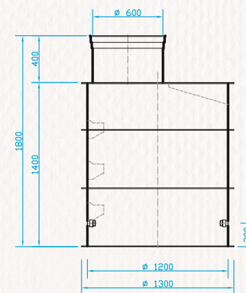
WATER SHAFT - OVAL 4 1200x900x1800 mm
