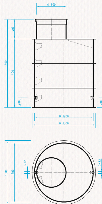
WATER SHAFT - CIRCULAR 3 \varnothing 1200 \times 1800 mm
