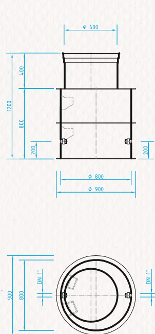
WATER SHAFT - CIRCULAR 1 \varnothing 800 \times 1200 mm
