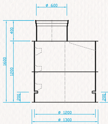
WATER SHAFT - OVAL 1 1200x900x1600 mm
