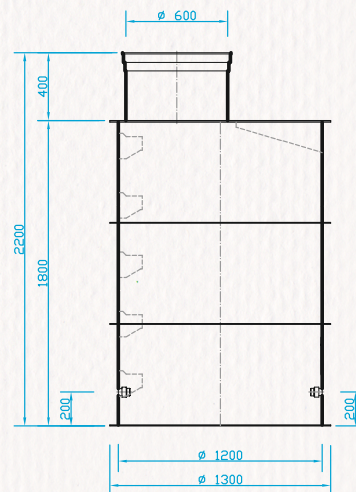
WATER SHAFT - OVAL 3 1200x900x2200 mm
