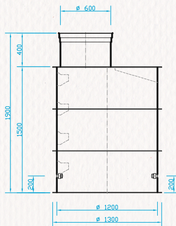
WATER SHAFT - OVAL 2 1200x900x1900 mm
